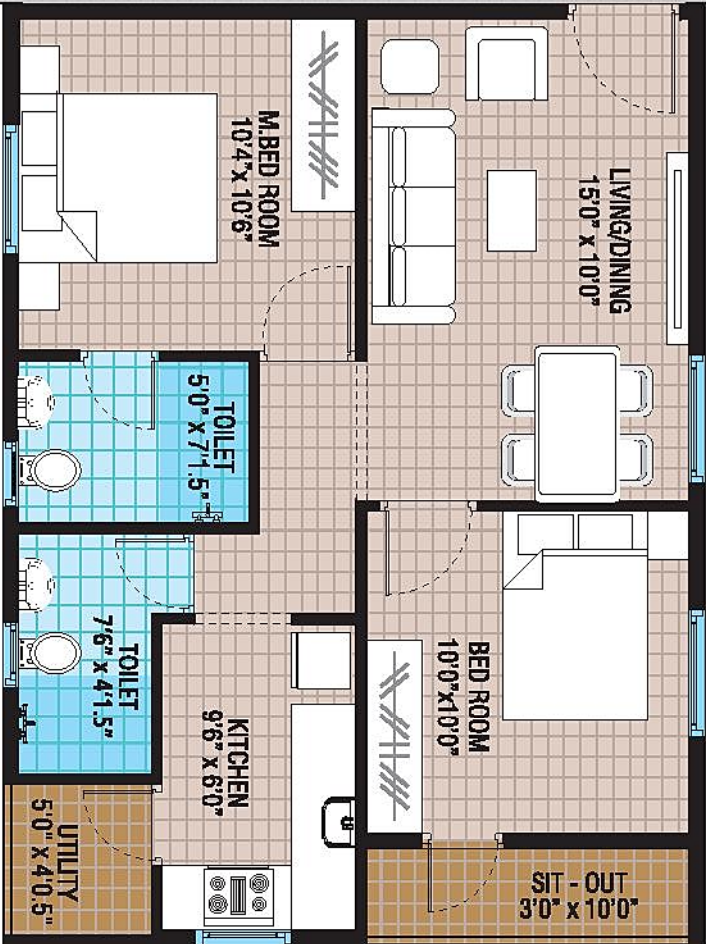
TYPE B - AREA - 800 SFT
